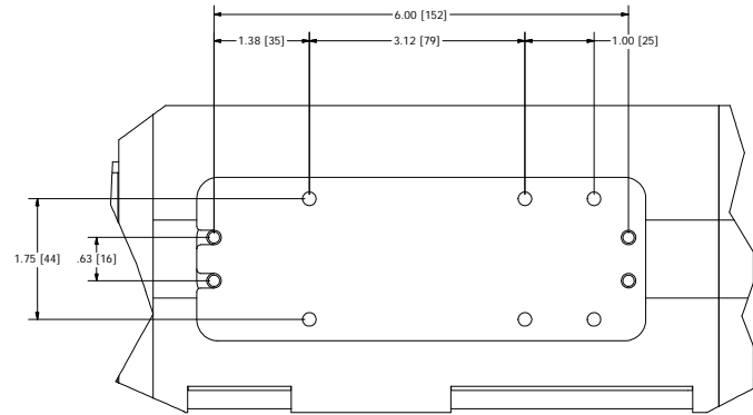
DETAIL A SCALE 1 : 1 Optional Universal Mounting Base Plate PN 7000-243 2 Required
